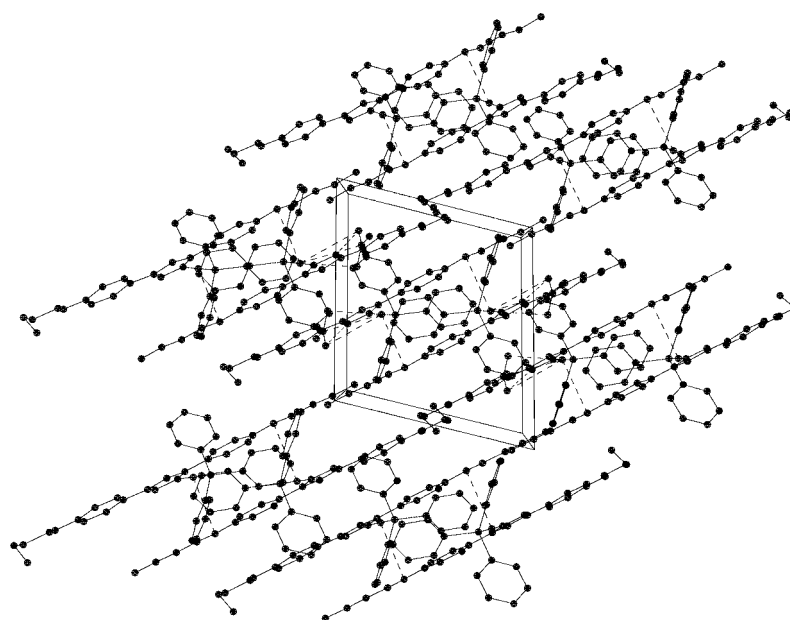
Figure 3. Molecular packing of 5 through c axis
