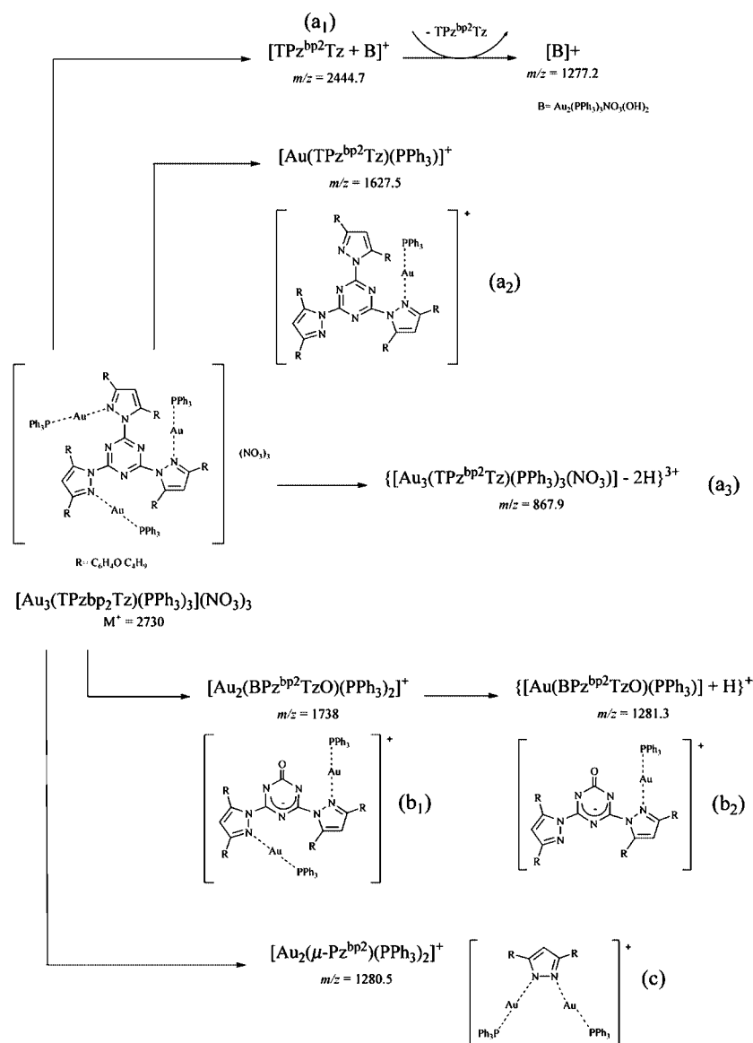
Figure 4. Fragmentation scheme for the complex [Au_3(TPz^{bp2}Tz)(PPh_3)_3](NO_3)_3 9 ; symbols (a), (b), and (c) indicate: (a) fragments containing the TPz^{bp2}Tz ligand, (b) fragments containing the hydrolysed TPz^{bp2}Tz ligand ( BPz^{bp2}TzO ), and (c) side product
