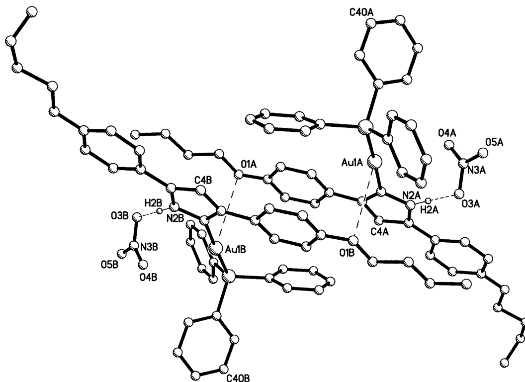
Figure 2. Molecular structure of 5 showing the dimeric unit through Au...O intermolecular bonds
