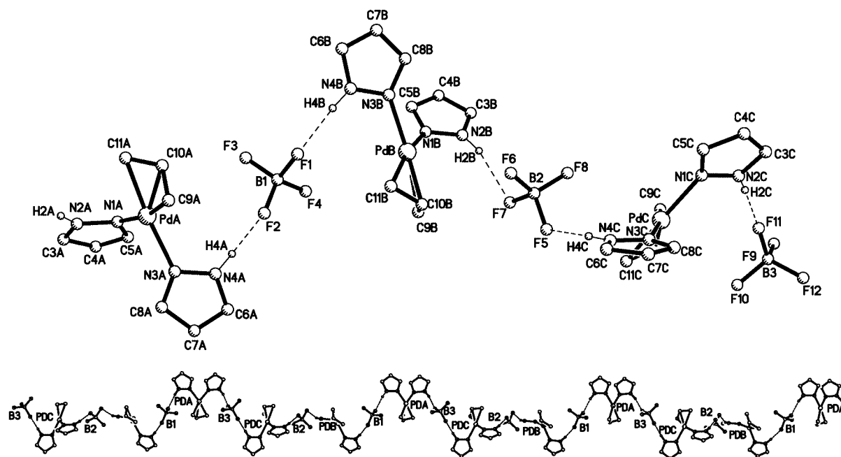
Figure 1. (top) Asymmetric unit of 4 with the atomic numbering scheme; (bottom) View of the helical distribution of 4 along c axis; substituents on pyrazole in both pictures are omitted for clarity
